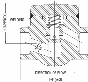
WELDED DESIGN
